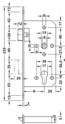
Forend width 20 mm for rebated doors
